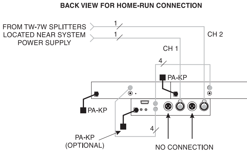
FIGURE 12. Typical Remote Binaural Speaker Station. This example is similar to the one on the previous page, except that each channel is heard in a separate speaker. Make sure the internal DIP switches are set for binaural speaker operation as described on page 9. As in the previous example, a PA-KP local power supply is required for each SPK2000 speaker, but is optional for the US2002.
