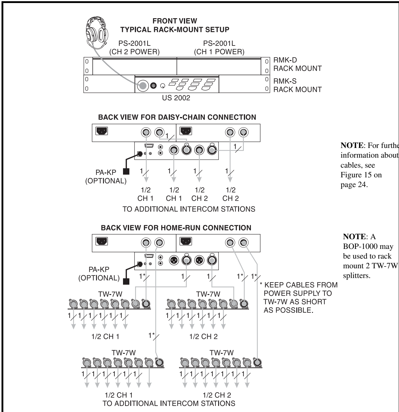
FIGURE 9. US2002 Headset Station Configuration with 2 Power Supplies. In this configuration, the PS2001L Combine/Isolate switches are set to the Combine position. With this setting all intercom stations connected to the one PS2001L are combined on intercom channel 1 and all intercom stations connected to the other PS2001L are combined on channel 2. Typically, a headset is connected to the front panel of the US2002, and the US2002 dip switches are set to monaural operation (default setting) so that both intercom channels are heard in the monaural headphones (binaural headphone operation is not supported). The PA-KP local power supply is optional. When a PA-KP is connected, the US2002 automatically disconnects from system power. Since the US2002 is not drawing power from the intercom system, more system power is available for additional belt packs, etc.
