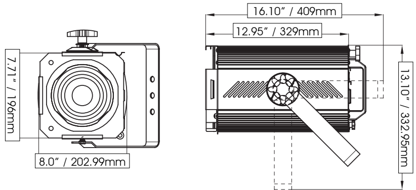
ELED Fresnel 100WW Dimensions
